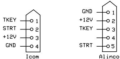
RADIO CONNECTORS
